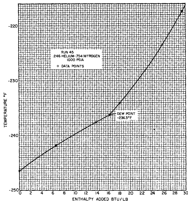
Fig. 7. Differential latent heat of a helium-nitrogen mixture.
